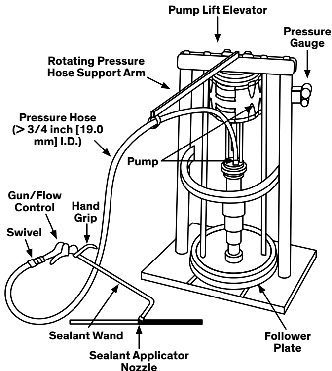
Figure 5 – Extrusion Pump
