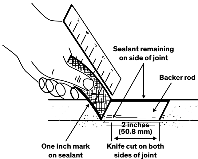
Figure 1 – Standard Field Adhesion Hand Pull Test
