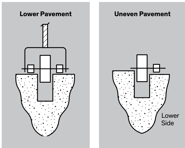
Figure 4 – Backer Rod Installation Tools
