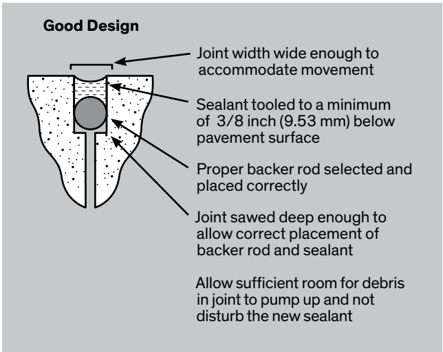
Figure 2 – Joint Design Considerations: DOWSIL™ 888 Silicone Joint Sealant
